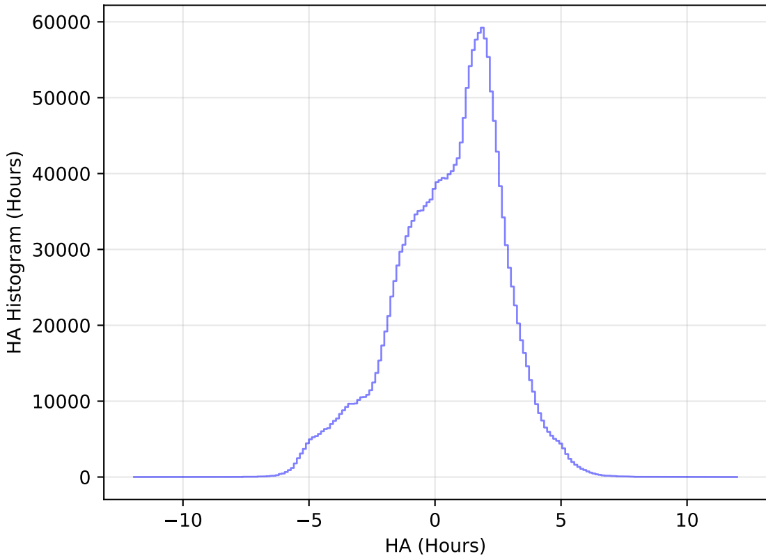
no_high_blob_v3.3_10yrs All sky all bands: HA Histogram
