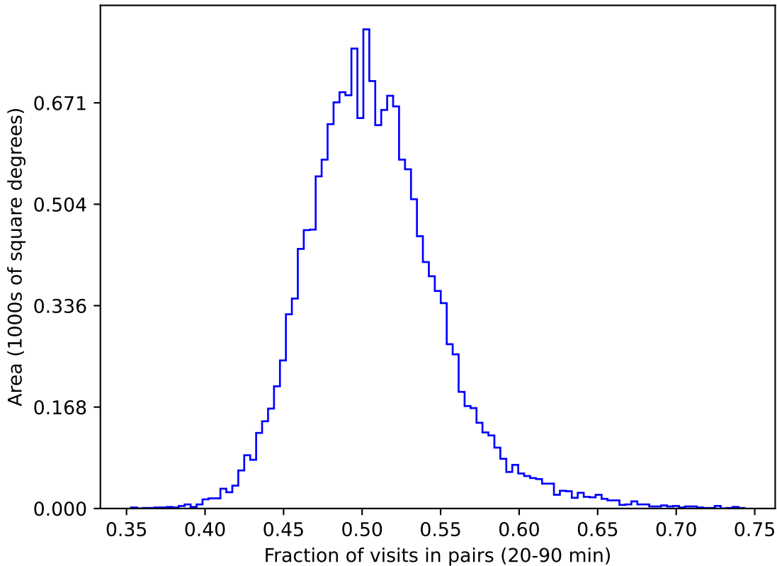
no_high_blob_v3.3_10yrs gri WFD: Fraction of visits in pairs (20-90 min)
