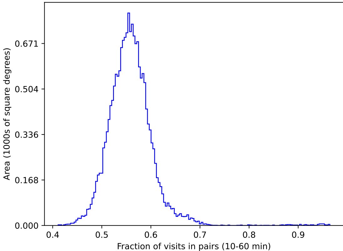
no_high_blob_v3.3_10yrs gri WFD: Fraction of visits in pairs (10-60 min)
