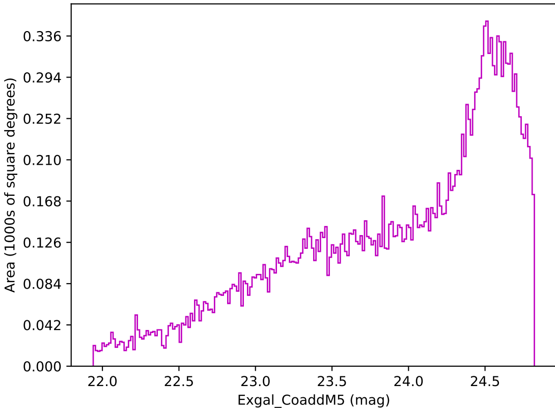
no_high_blob_v3.3_10yrs Yr 3-4 z band: Exgal_CoaddM5
