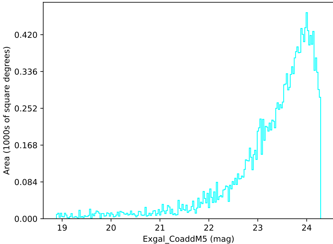
no_high_blob_v3.3_10yrs Yr 3-4 u band: Exgal_CoaddM5
