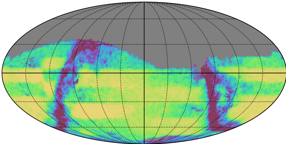
no_high_blob_v3.3_10yrs Yr 3-4 r band: Exgal_CoaddM5
