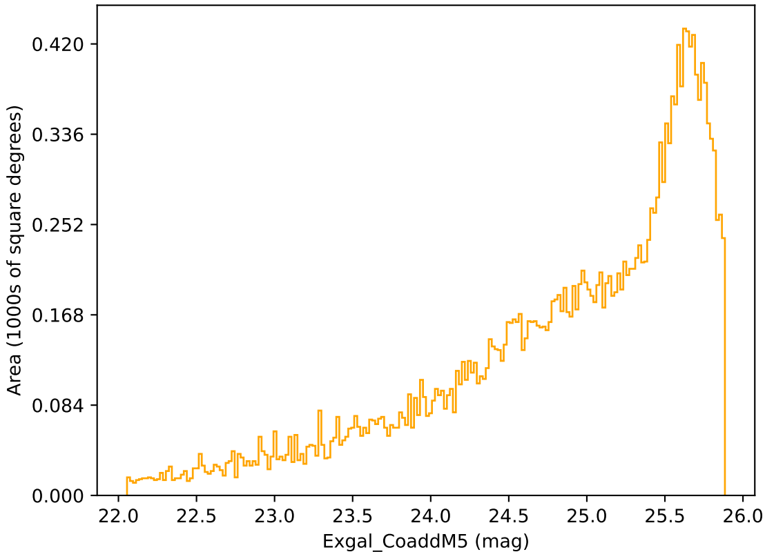
no_high_blob_v3.3_10yrs Yr 3-4 r band: Exgal_CoaddM5
