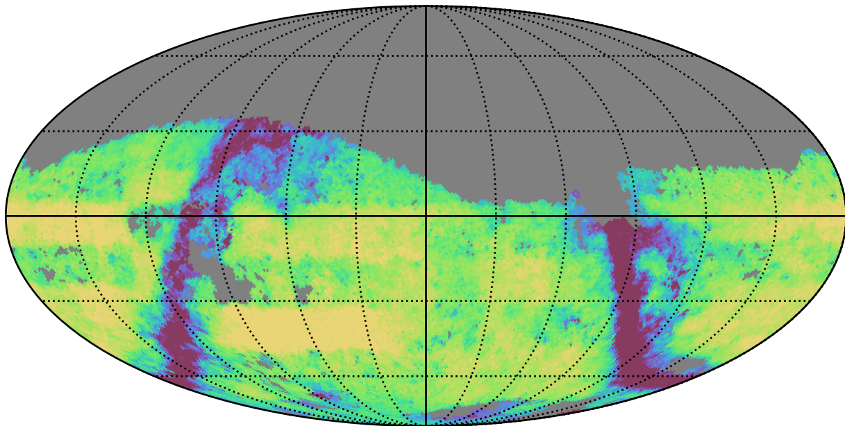
no_high_blob_v3.3_10yrs Yr 3-4 g band: Exgal_CoaddM5
