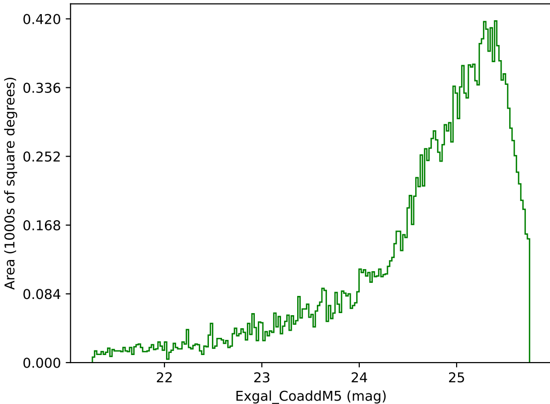
no_high_blob_v3.3_10yrs Yr 3-4 g band: Exgal_CoaddM5
