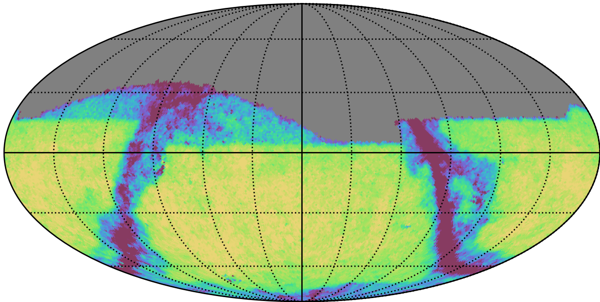
no_high_blob_v3.3_10yrs Yr 1 z band: Exgal_CoaddM5
