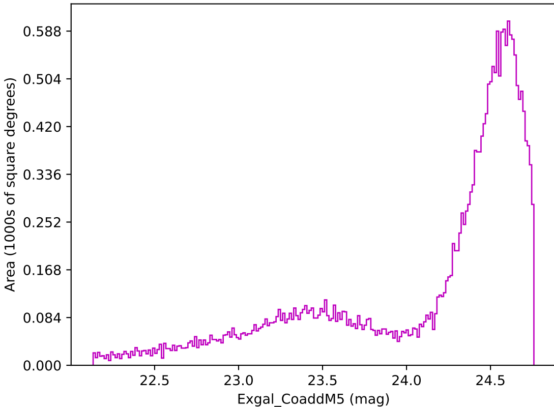
no_high_blob_v3.3_10yrs Yr 1 z band: Exgal_CoaddM5
