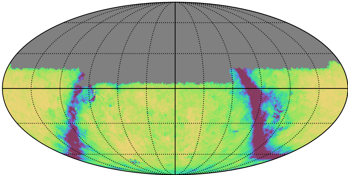
no_high_blob_v3.3_10yrs Yr 1 u band: Exgal_CoaddM5
