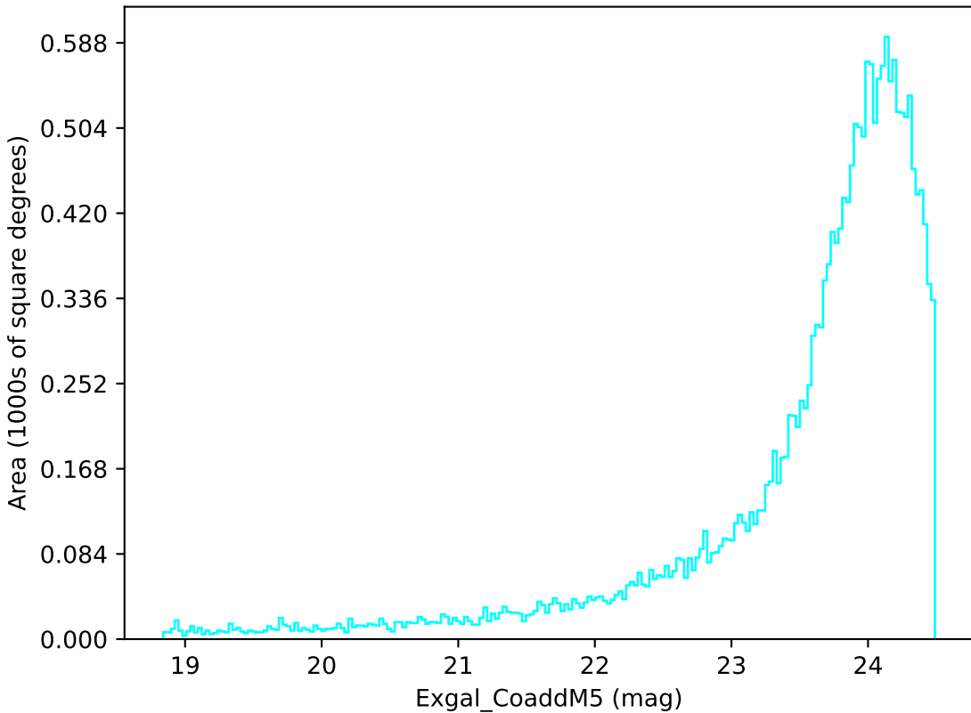
no_high_blob_v3.3_10yrs Yr 1 u band: Exgal_CoaddM5
