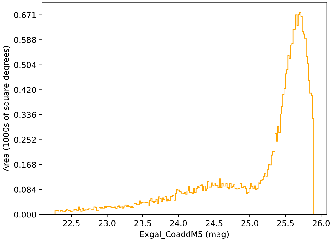
no_high_blob_v3.3_10yrs Yr 1 r band: Exgal_CoaddM5
