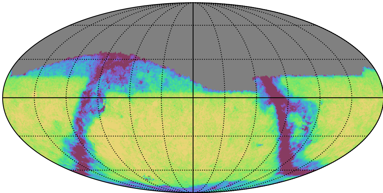
no_high_blob_v3.3_10yrs Yr 1 i band: Exgal_CoaddM5
