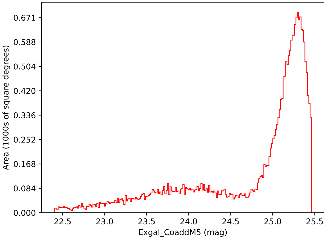
no_high_blob_v3.3_10yrs Yr 1 i band: Exgal_CoaddM5
