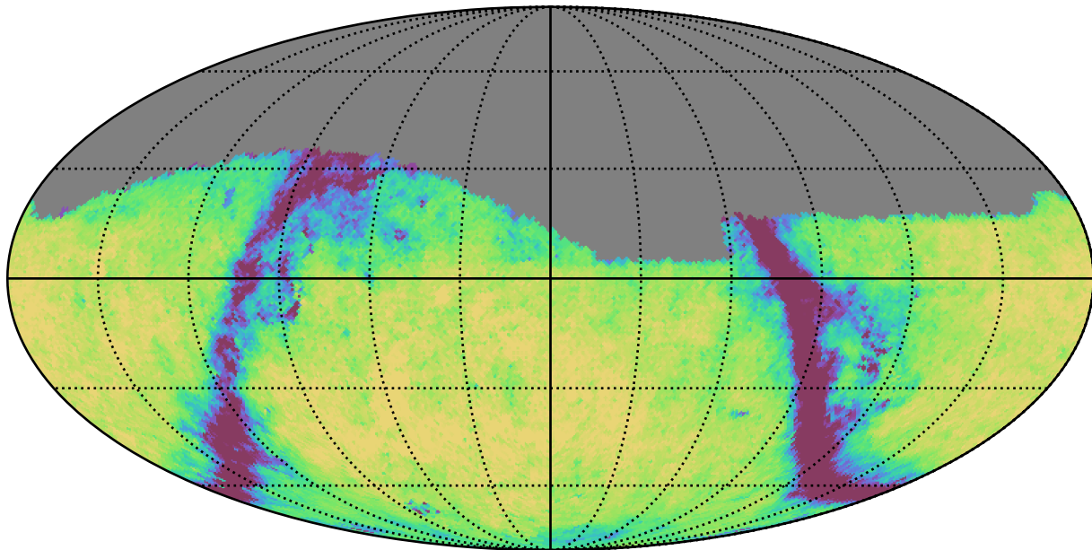
no_high_blob_v3.3_10yrs Yr 1 g band: Exgal_CoaddM5
