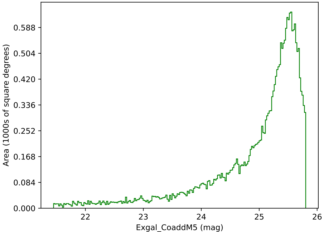
no_high_blob_v3.3_10yrs Yr 1 g band: Exgal_CoaddM5
