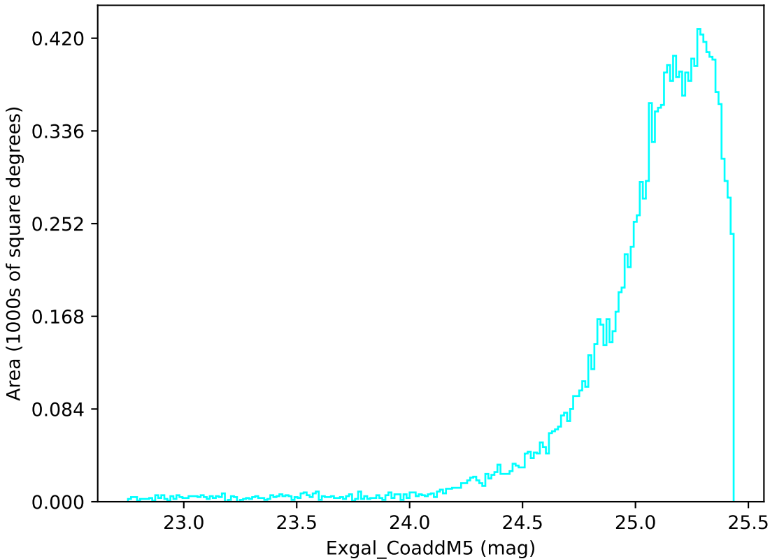
no_high_blob_v3.3_10yrs WFD u band: Exgal_CoaddM5
