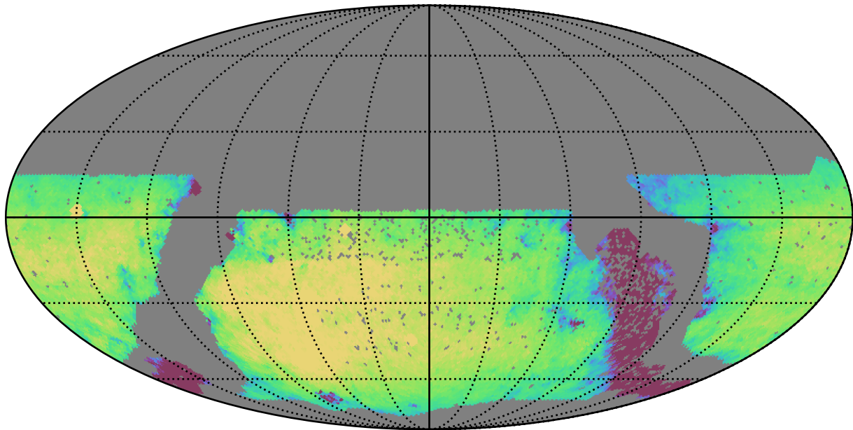
no_high_blob_v3.3_10yrs WFD r band: Exgal_CoaddM5
