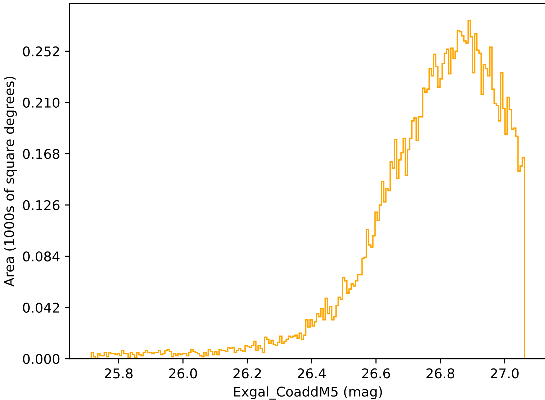
no_high_blob_v3.3_10yrs WFD r band: Exgal_CoaddM5
