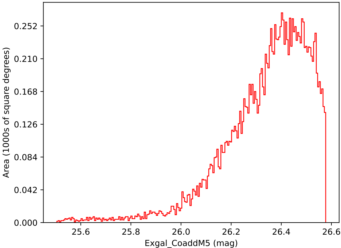
no_high_blob_v3.3_10yrs WFD i band: Exgal_CoaddM5
