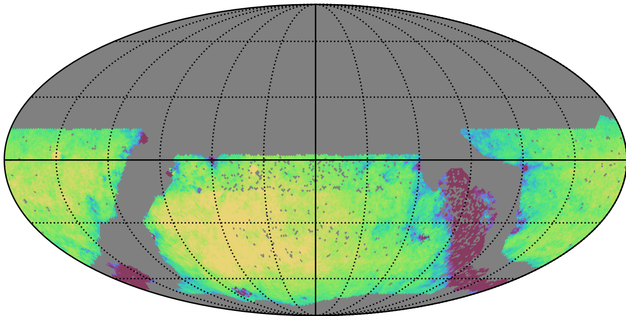
no_high_blob_v3.3_10yrs WFD g band: Exgal_CoaddM5
