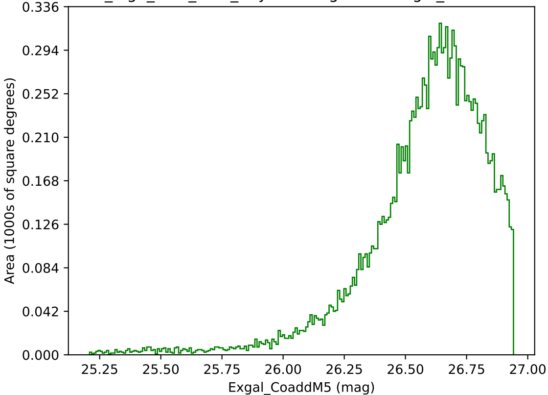
no_high_blob_v3.3_10yrs WFD g band: Exgal_CoaddM5
