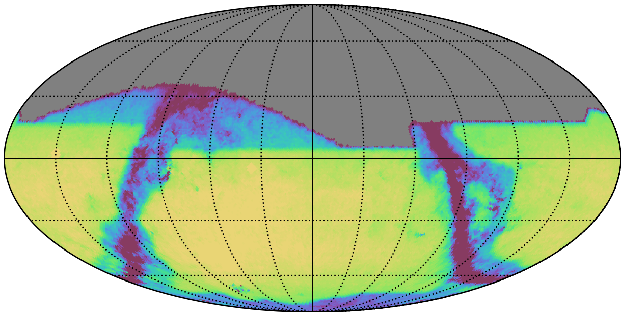
no_high_blob_v3.3_10yrs All sky z band: Exgal_CoaddM5
