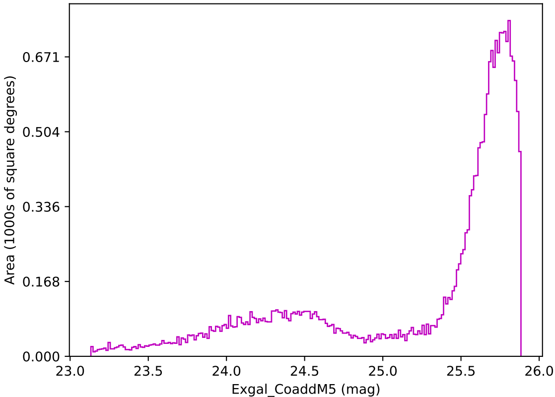
no_high_blob_v3.3_10yrs All sky z band: Exgal_CoaddM5
