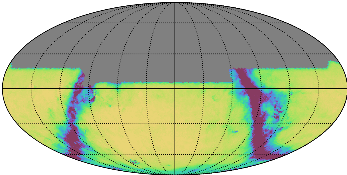
no_high_blob_v3.3_10yrs All sky u band: Exgal_CoaddM5
