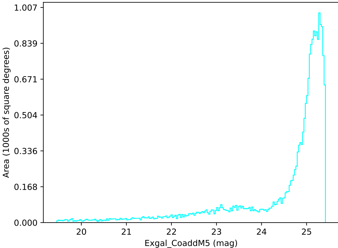
no_high_blob_v3.3_10yrs All sky u band: Exgal_CoaddM5
