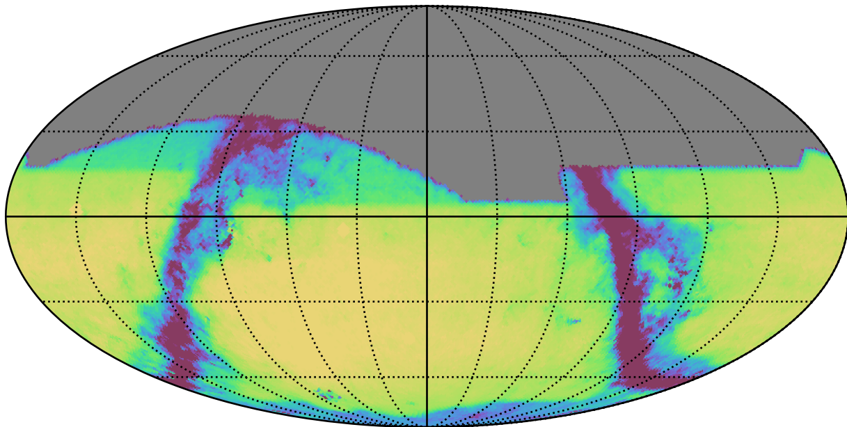
no_high_blob_v3.3_10yrs All sky r band: Exgal_CoaddM5
