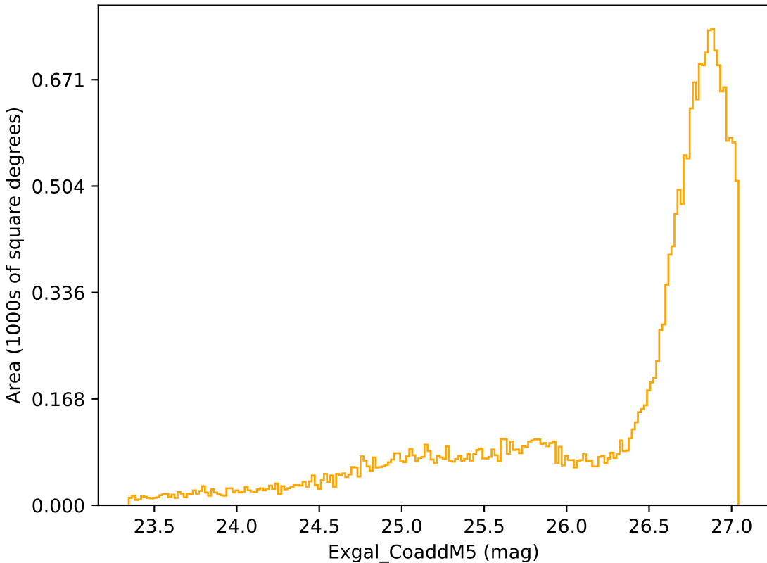
no_high_blob_v3.3_10yrs All sky r band: Exgal_CoaddM5
