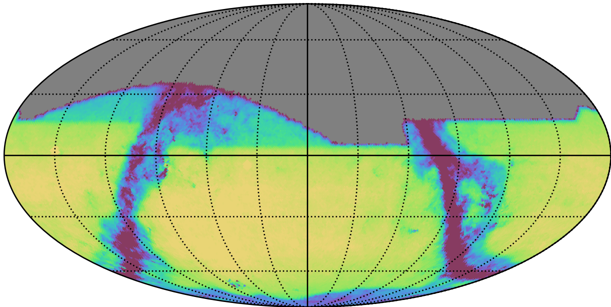
no_high_blob_v3.3_10yrs All sky i band: Exgal_CoaddM5
