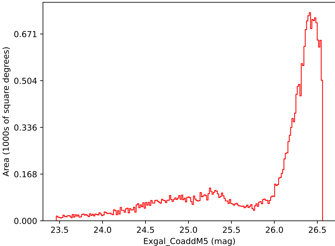
no_high_blob_v3.3_10yrs All sky i band: Exgal_CoaddM5
