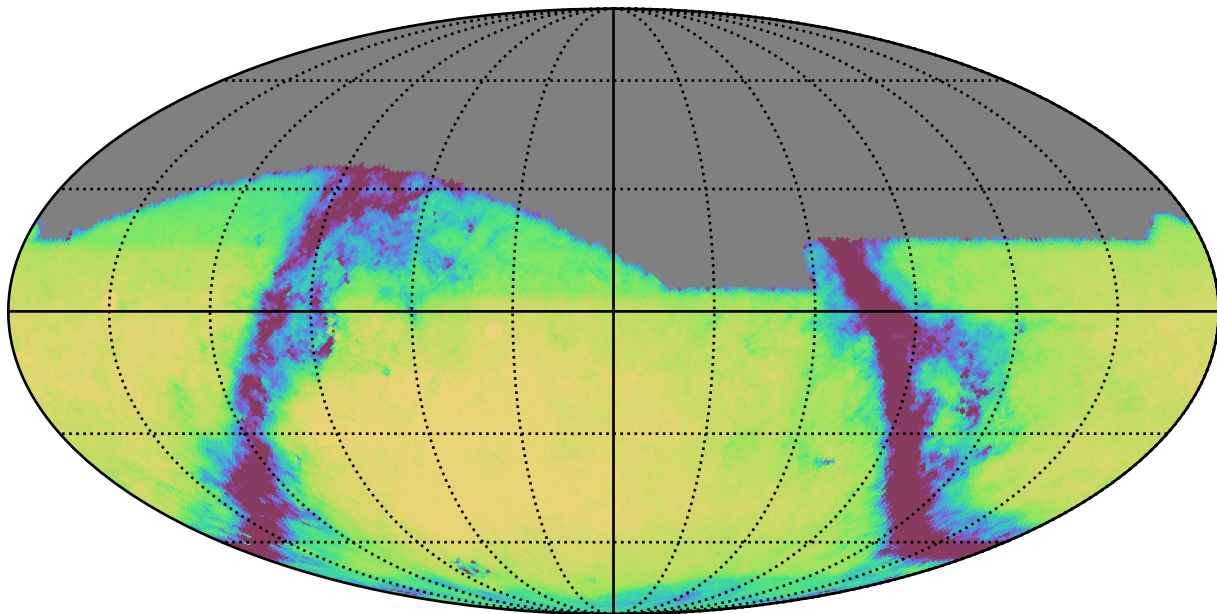
no_high_blob_v3.3_10yrs All sky g band: Exgal_CoaddM5
