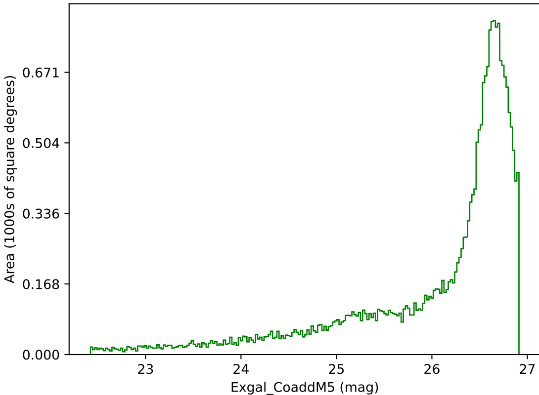
no_high_blob_v3.3_10yrs All sky g band: Exgal_CoaddM5
