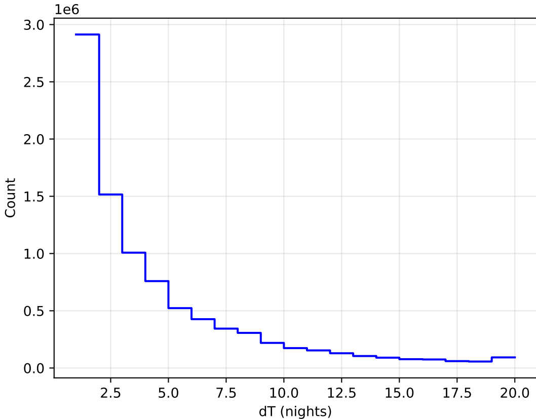
no_high_blob_v3.3_10yrs All sky all bands: DeltaNight Histogram
