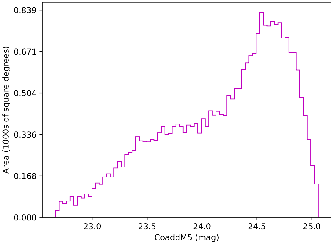
no_high_blob_v3.3_10yrs Yr 3-4 z band: CoaddM5
