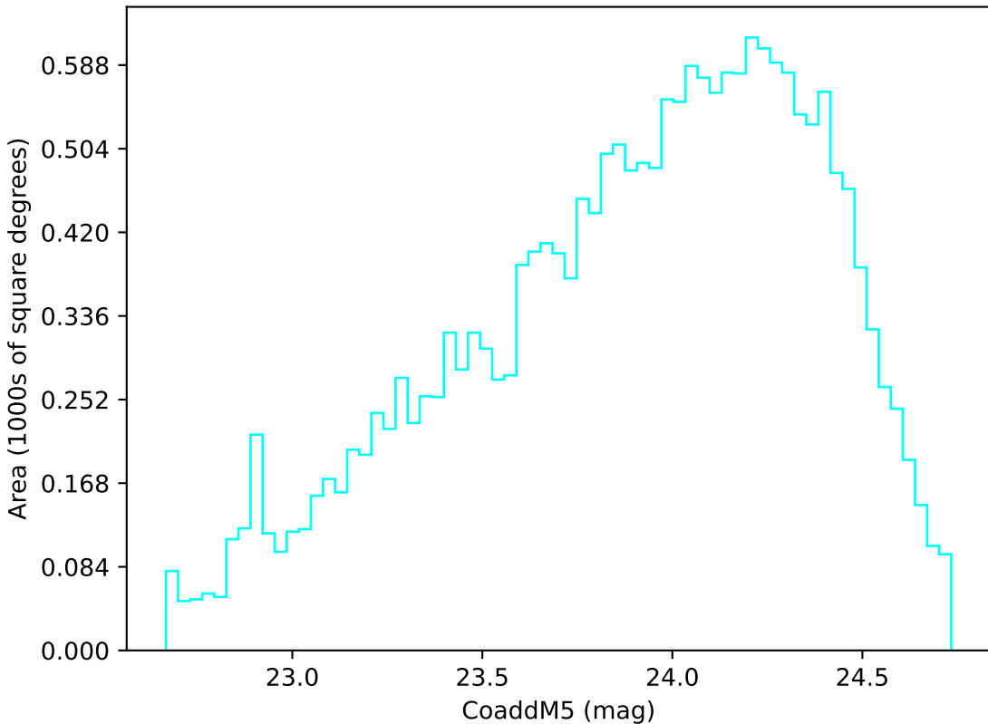
no_high_blob_v3.3_10yrs Yr 3-4 u band: CoaddM5
