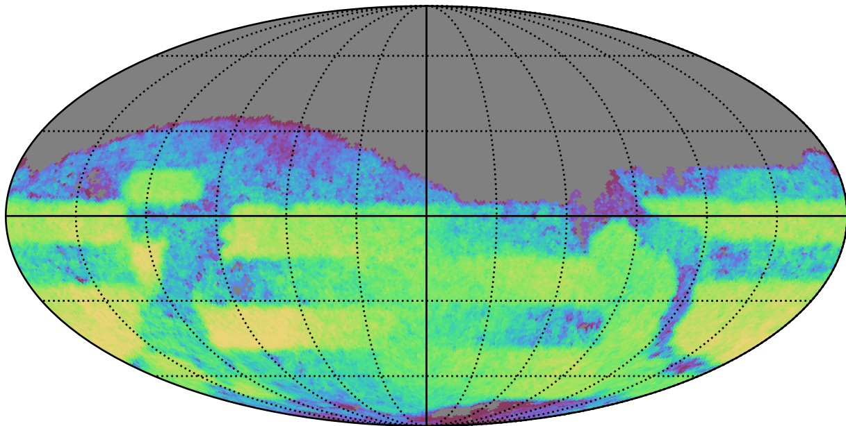
no_high_blob_v3.3_10yrs Yr 3-4 r band: CoaddM5
