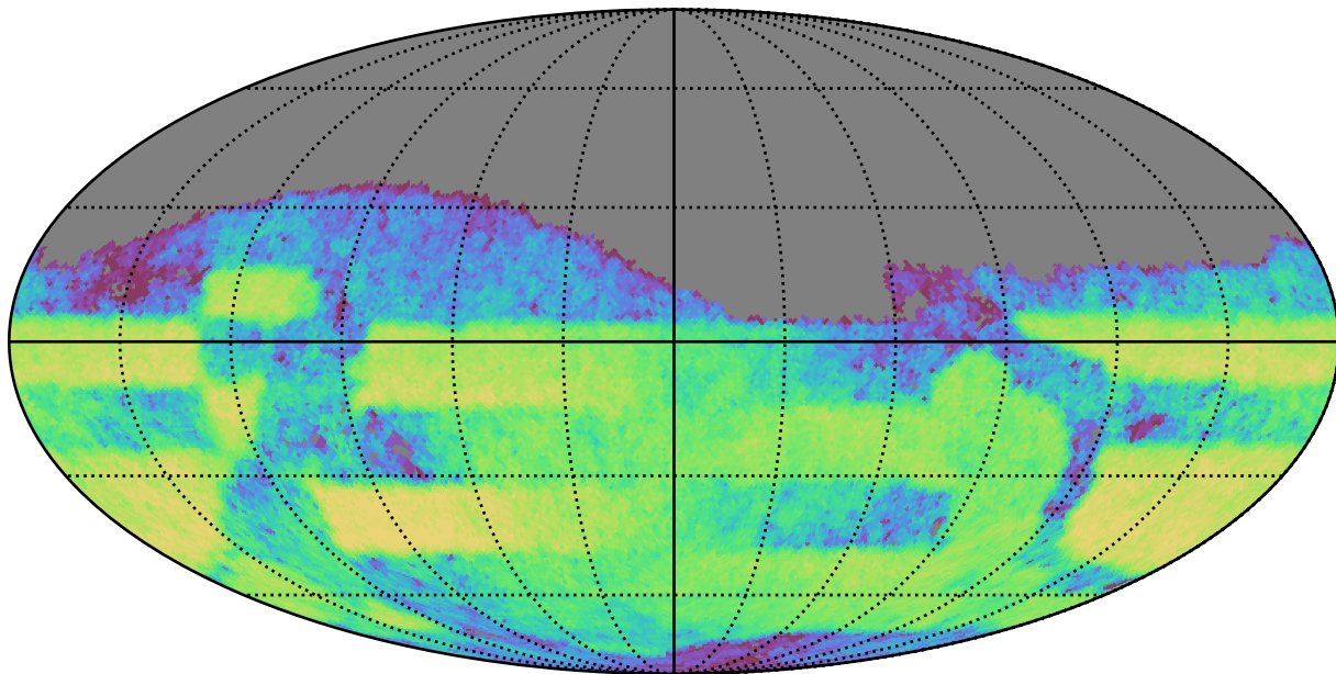
no_high_blob_v3.3_10yrs Yr 3-4 i band: CoaddM5
