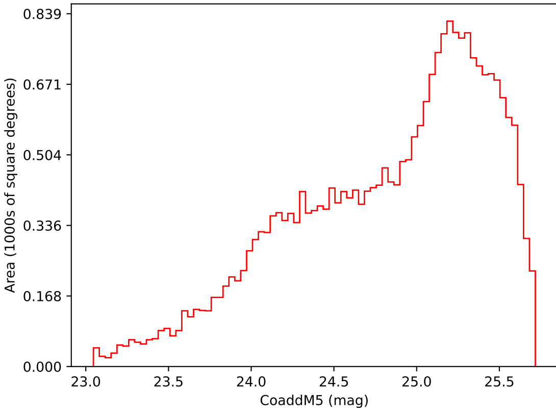
no_high_blob_v3.3_10yrs Yr 3-4 i band: CoaddM5
