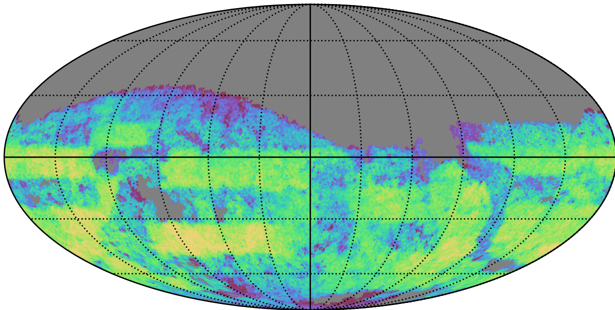
no_high_blob_v3.3_10yrs Yr 3-4 g band: CoaddM5
