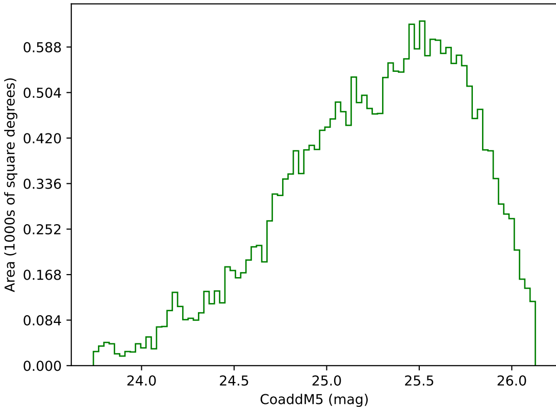
no_high_blob_v3.3_10yrs Yr 3-4 g band: CoaddM5
