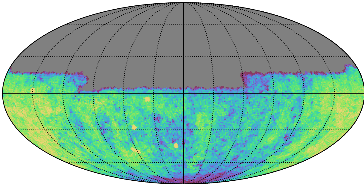
no_high_blob_v3.3_10yrs Yr 1 u band: CoaddM5
