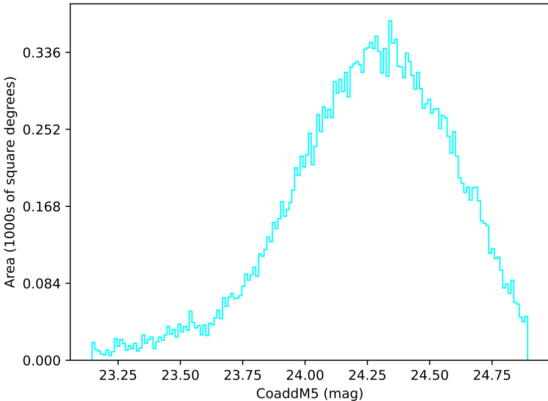
no_high_blob_v3.3_10yrs Yr 1 u band: CoaddM5
