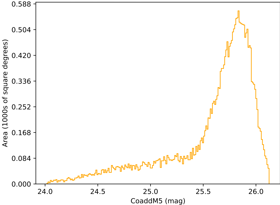
no_high_blob_v3.3_10yrs Yr 1 r band: CoaddM5
