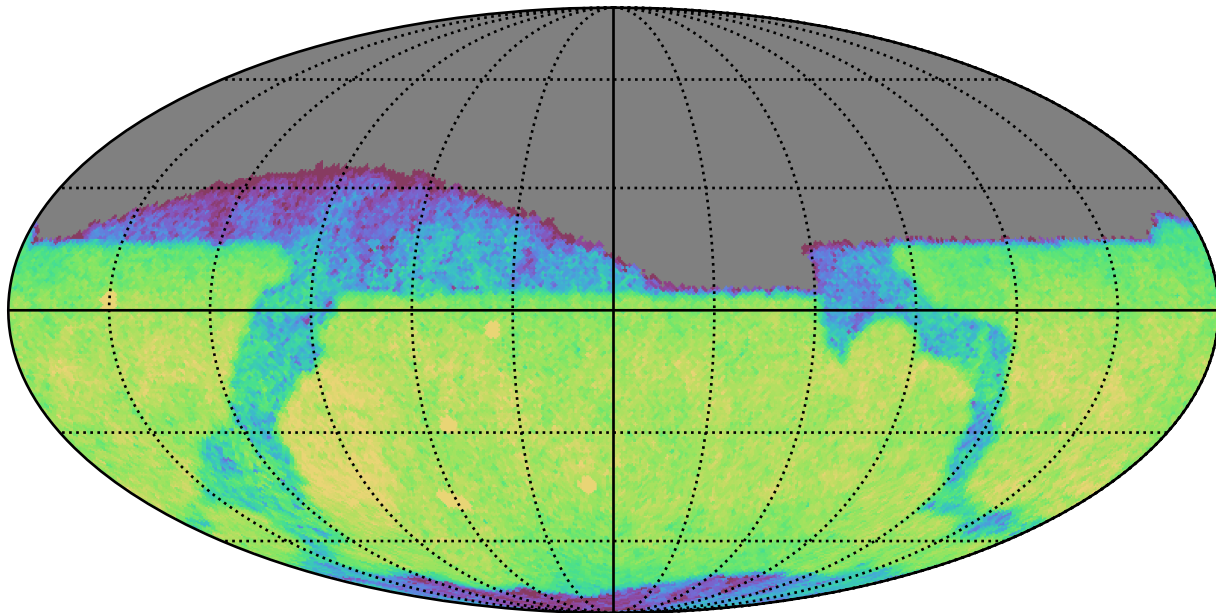
no_high_blob_v3.3_10yrs Yr 1 i band: CoaddM5
