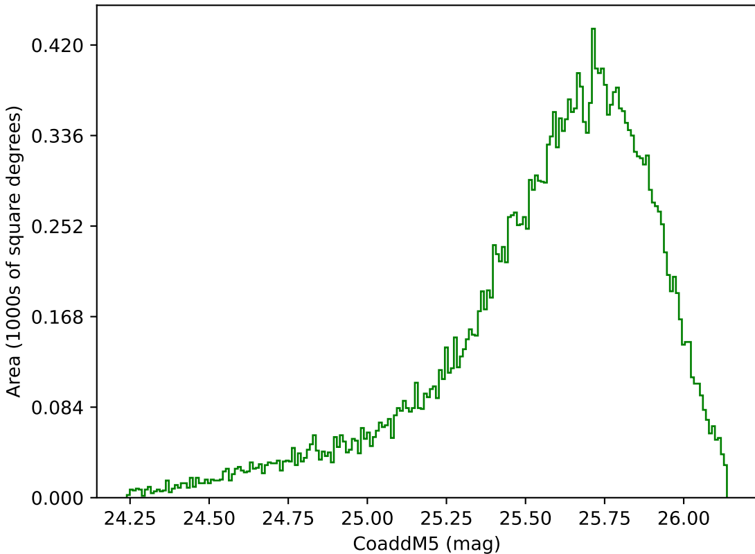
no_high_blob_v3.3_10yrs Yr 1 g band: CoaddM5
