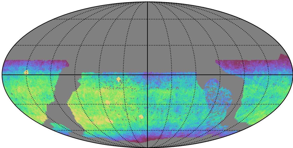
no_high_blob_v3.3_10yrs WFD z band: CoaddM5
