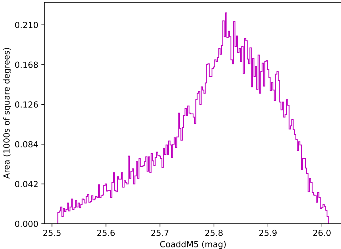
no_high_blob_v3.3_10yrs WFD z band: CoaddM5
