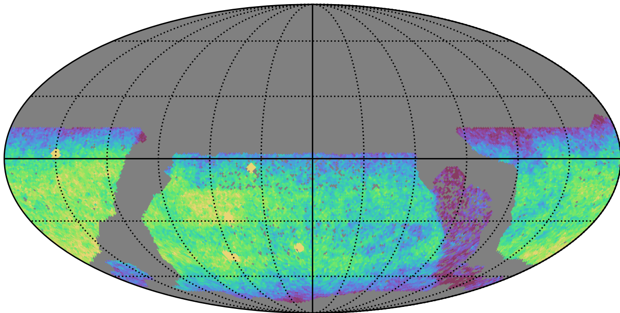
no_high_blob_v3.3_10yrs WFD u band: CoaddM5
